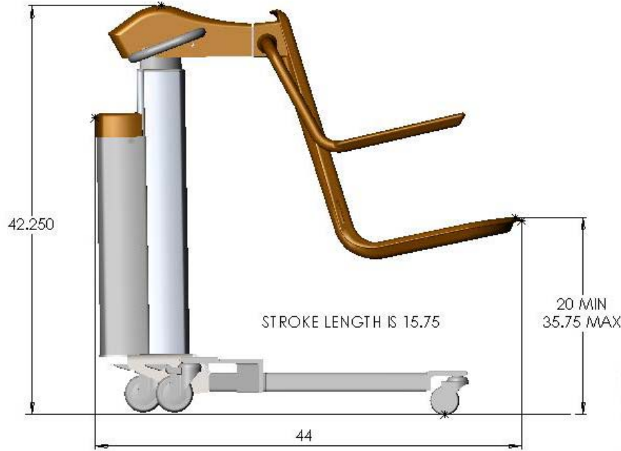
PENNER MFG CO. ELITE TRANSFER DIMENSIONS
